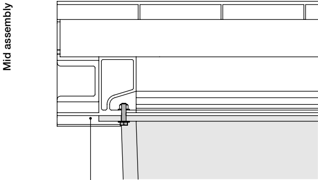
Heavy-duty float-flange attachment at side extrusion
