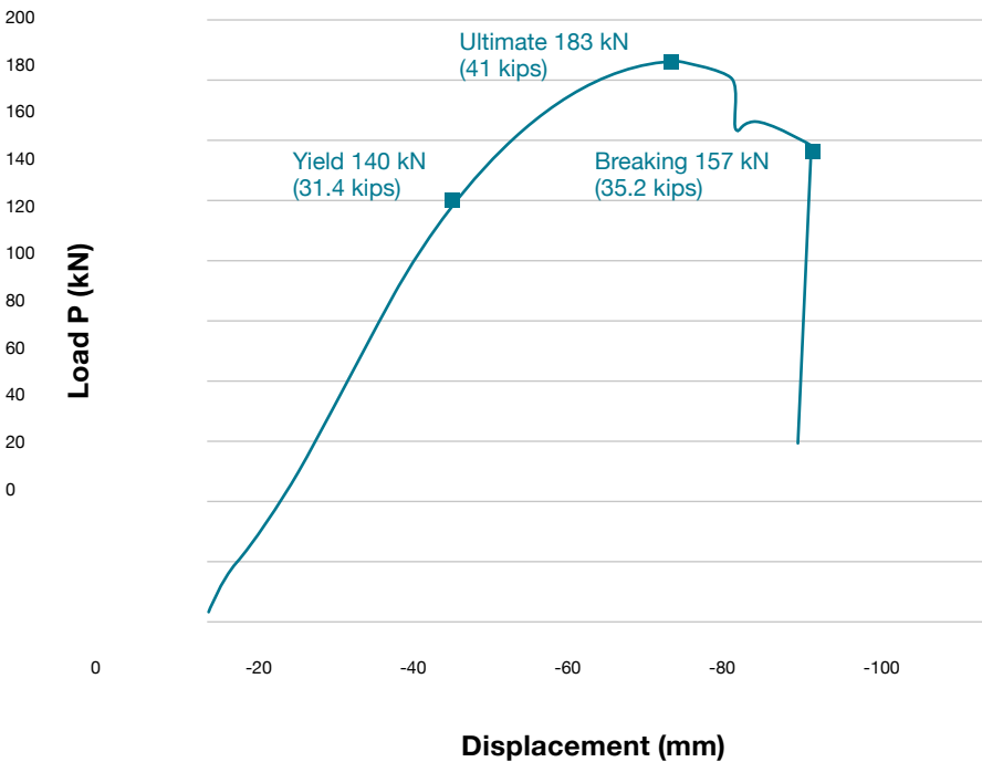
Total load (kN) vs. Displacement (mm)
